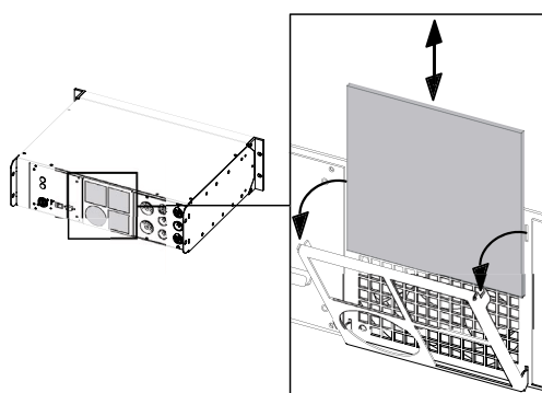
Fig. 22: D12 Fan filter exchange
