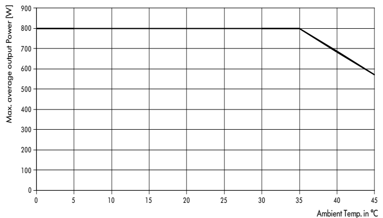
Fig. 23: Average maximum total output power vs. ambient temperature
