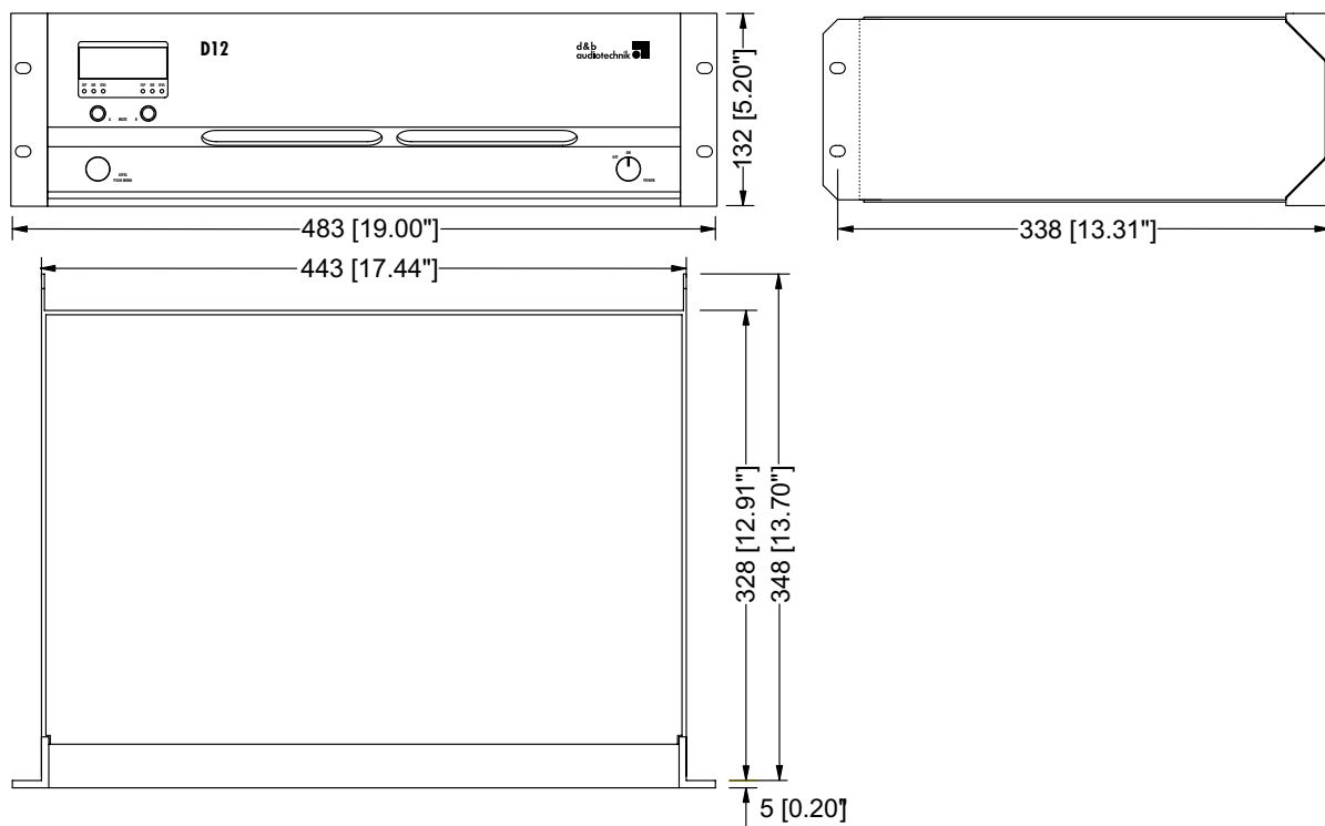
Fig. 26: D12 enclosure dimensions in mm [inch]
