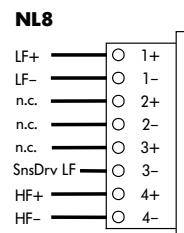
Fig. 20: Loudspeaker pin assignments and equivalents
