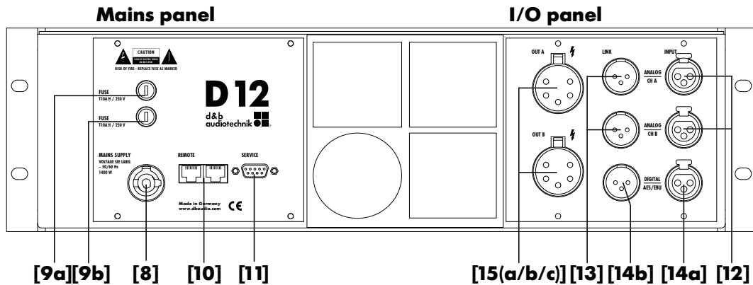
Fig. 8: D12 Connections
